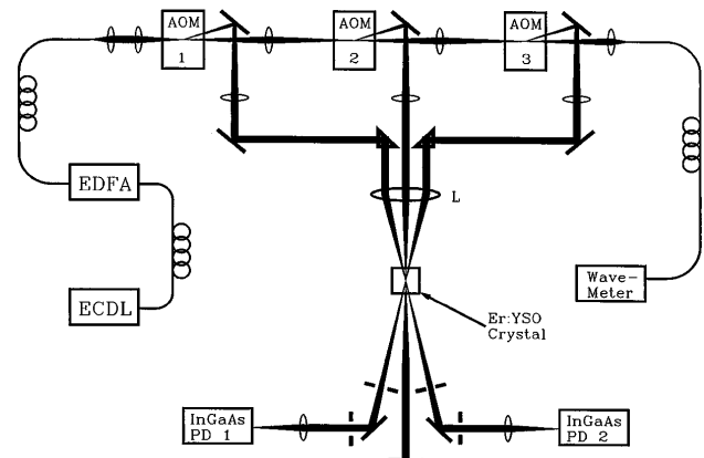
Fig. 2. Schematic of the experimental apparatus used for address header decoding. An external-cavity diode laser (EC DL) operating at 1536 nm is amplified by an erbium-doped fiber amplifier (EDFA) and gated by three AOM's to produce spatially separated beams that are crossed and focused in the crystal by lens L. Stimulated photon echoes are detected on the two InGaAs photodiodes (InGaAs PD 1, PD 2).
