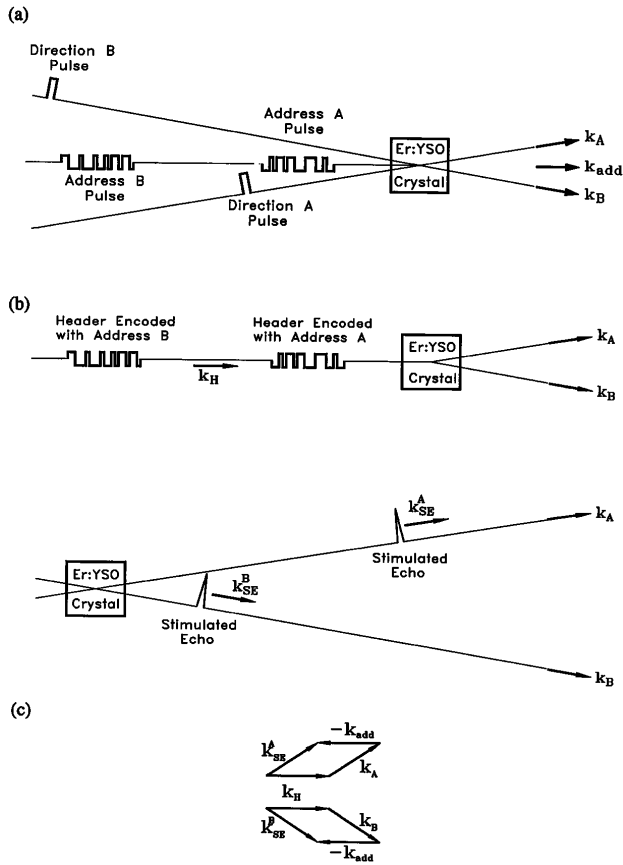
Fig. 1. (a) Temporal snapshot of the programming stage. For each header address, one spatial-spectral grating is stored in the crystal by a pair of programming pulses: a biphas-coded header address and a brief direction pulse. (b) Temporal snapshots of the processing stage. Headers coded with the addresses produce stimulated photon echoes in the spatial output channels that correspond to the directions programmed into the gratings by the brief direction pulses. (c) Phase-matching diagrams determining the wave vectors of the output stimulated photon echoes.
