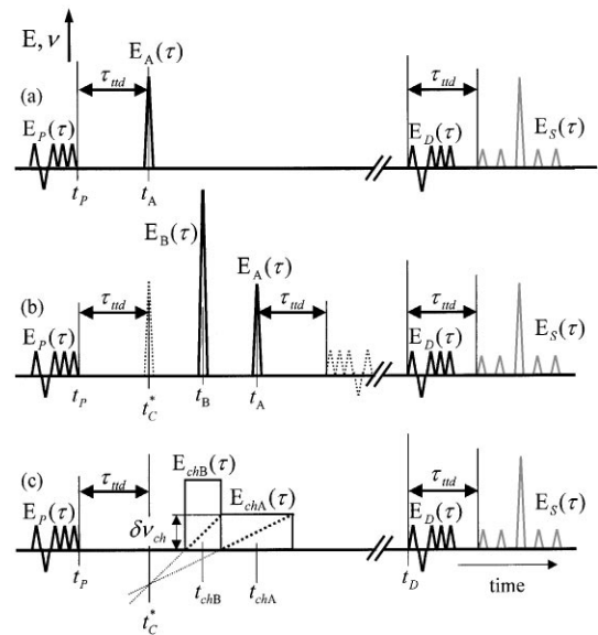
Fig. 1. Correlative signal processing using (a) traditional four-wave mixing with a single brief reference pulse, (b) six-wave mixing with two brief reference pulses, and (c) six-wave mixing with two chirped reference pulses.
